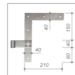
Winkelband Standard
