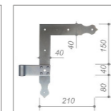
Winkelband Rustikal
