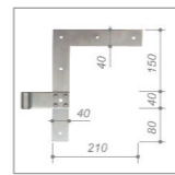
Winkelband Standard
