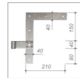
Winkelband Standard
