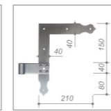
Winkelband Rustikal
